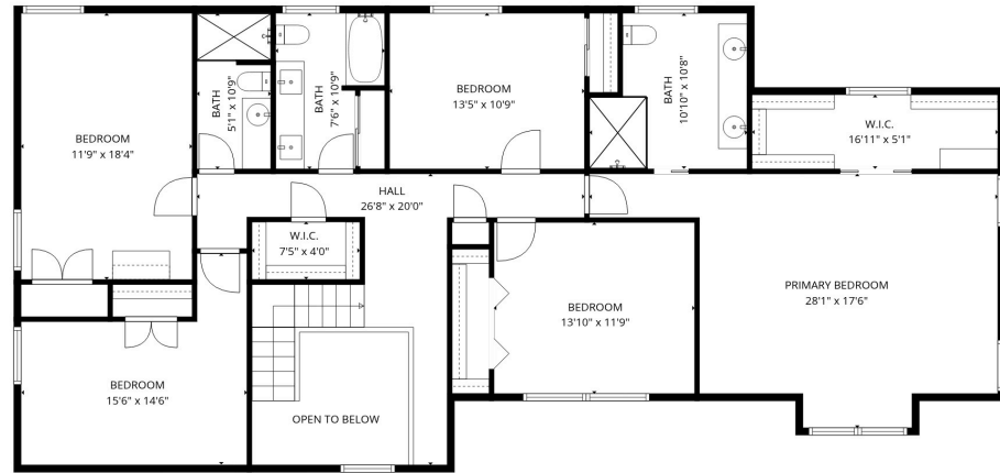
2nd floor
